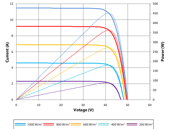
Current-Voltage & Power-Voltage Curve (450S)
